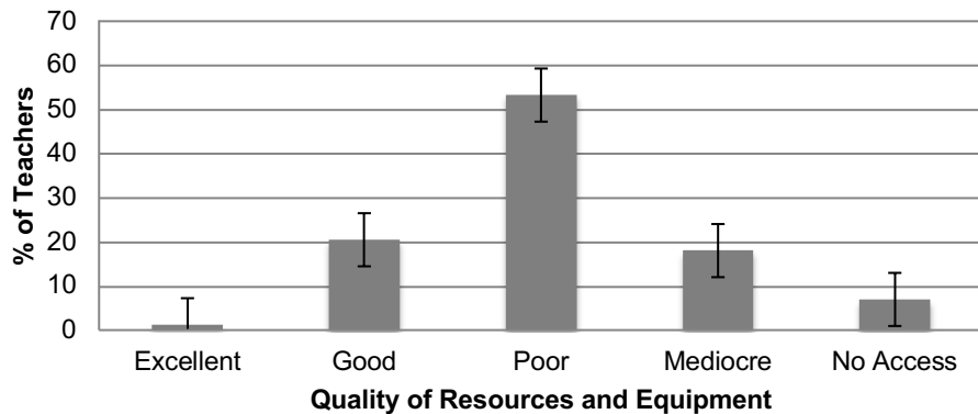
Figure 8. Perceived quality of the equipment and the resources used to teach astronomy (N = 244, uncertainty range \pm 6\% )
