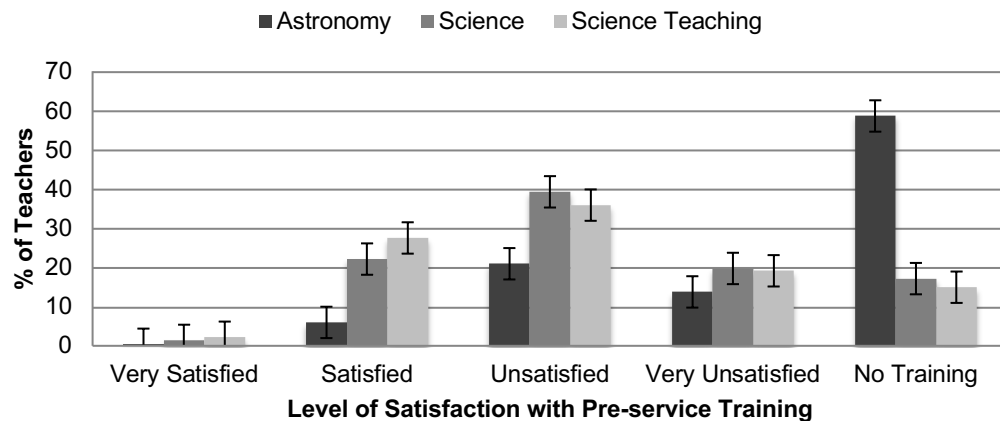
Figure 9. Level of satisfaction toward pre-service (university) training in astronomy, in science and in science teaching (N = 500, uncertainty range \pm 4\% )
