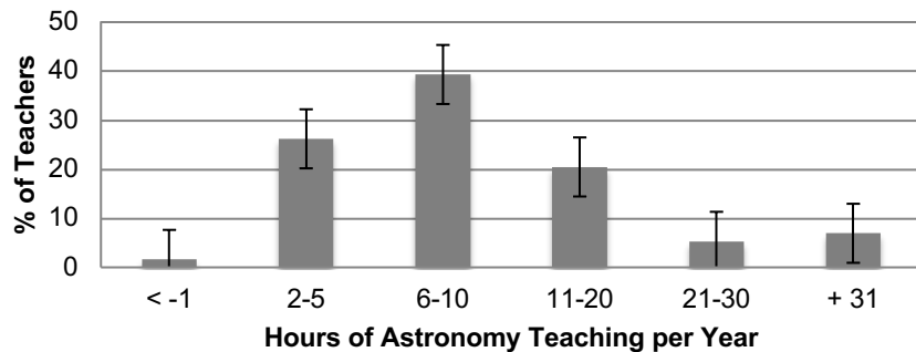
Figure 4. Number of hours of astronomy teaching per year (N = 244, uncertainty range \pm 6\% )
