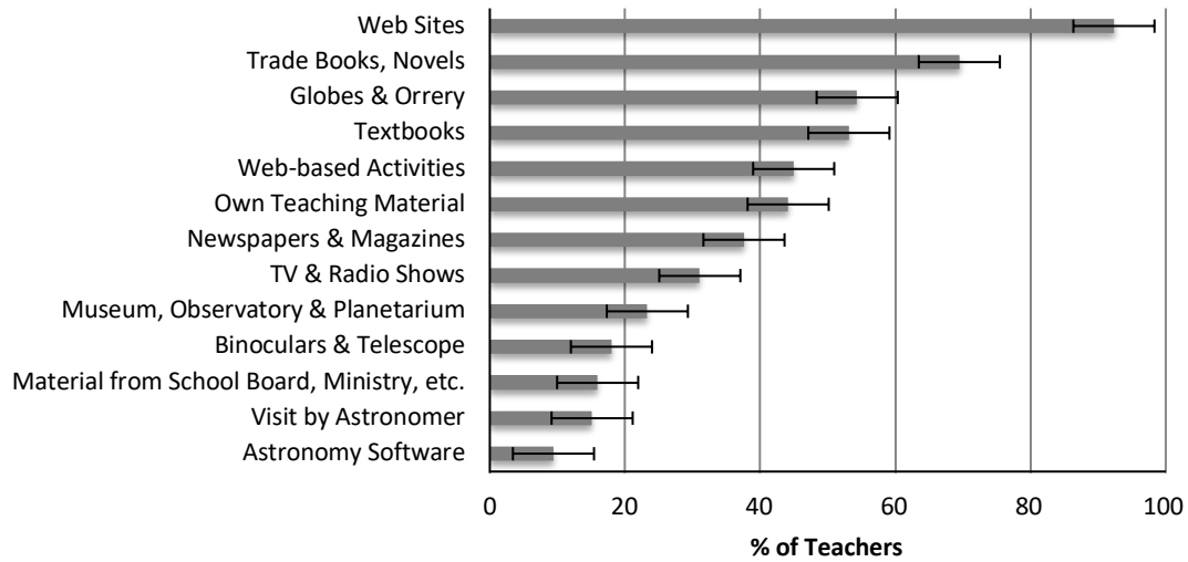
Figure 7. Materials used to teach astronomy (N = 244, uncertainty range \pm 6\% )
