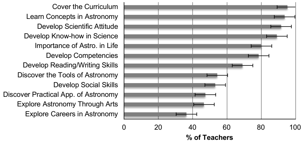
Figure 5. Aims and goals of astronomy teaching (N = 244, uncertainty range \pm 6\% )
