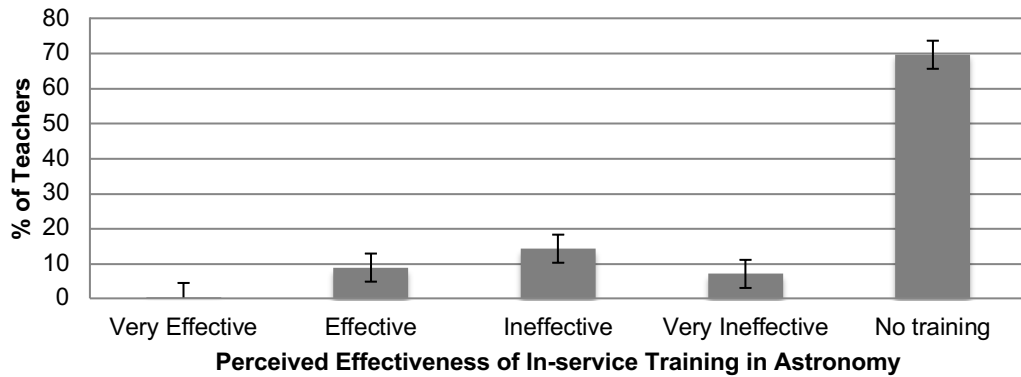
Figure 11. Perceived effectiveness of in-service training in astronomy (N = 500, uncertainty range \pm 4\% )
