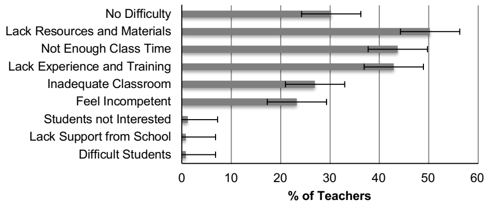
Figure 6. Sources of difficulty in teaching astronomy to the class (N = 244, uncertainty range \pm 6\% )
