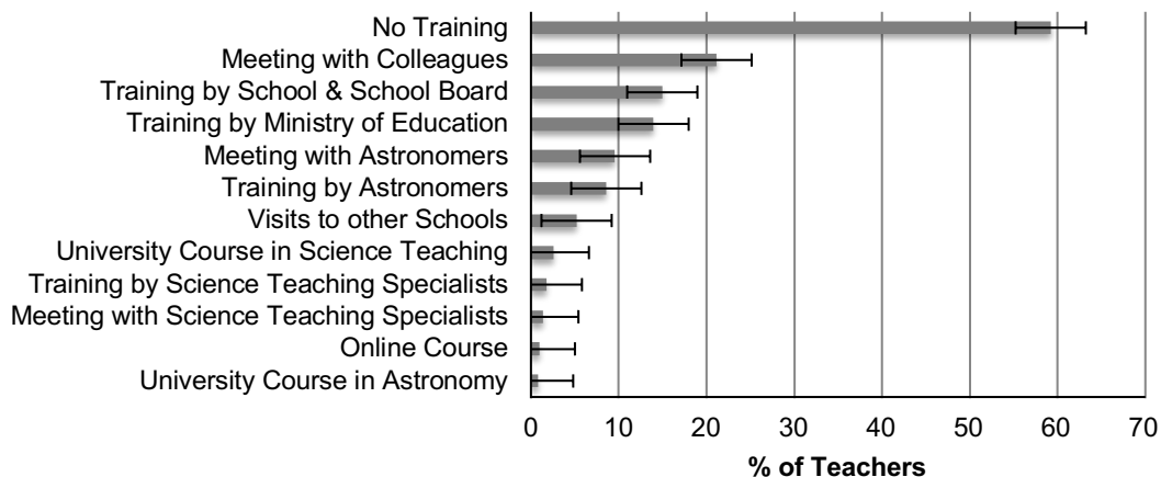
Figure 10. Type of in-service training in astronomy available to elementary teachers (N = 500, uncertainty range \pm 4\% )
