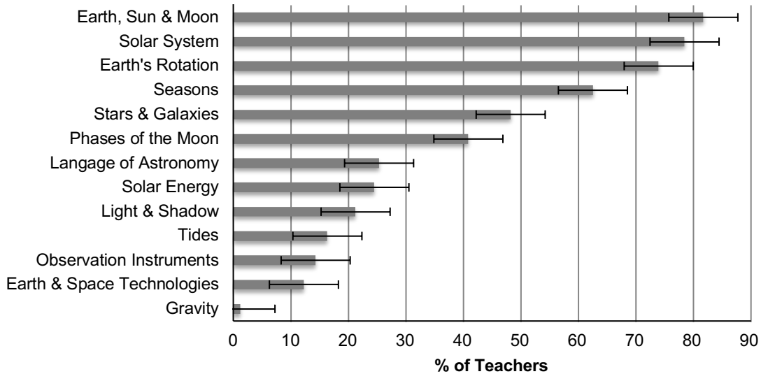
Figure 3. Astronomical topics taught in the elementary classroom (N = 244, uncertainty range \pm 6\% )
